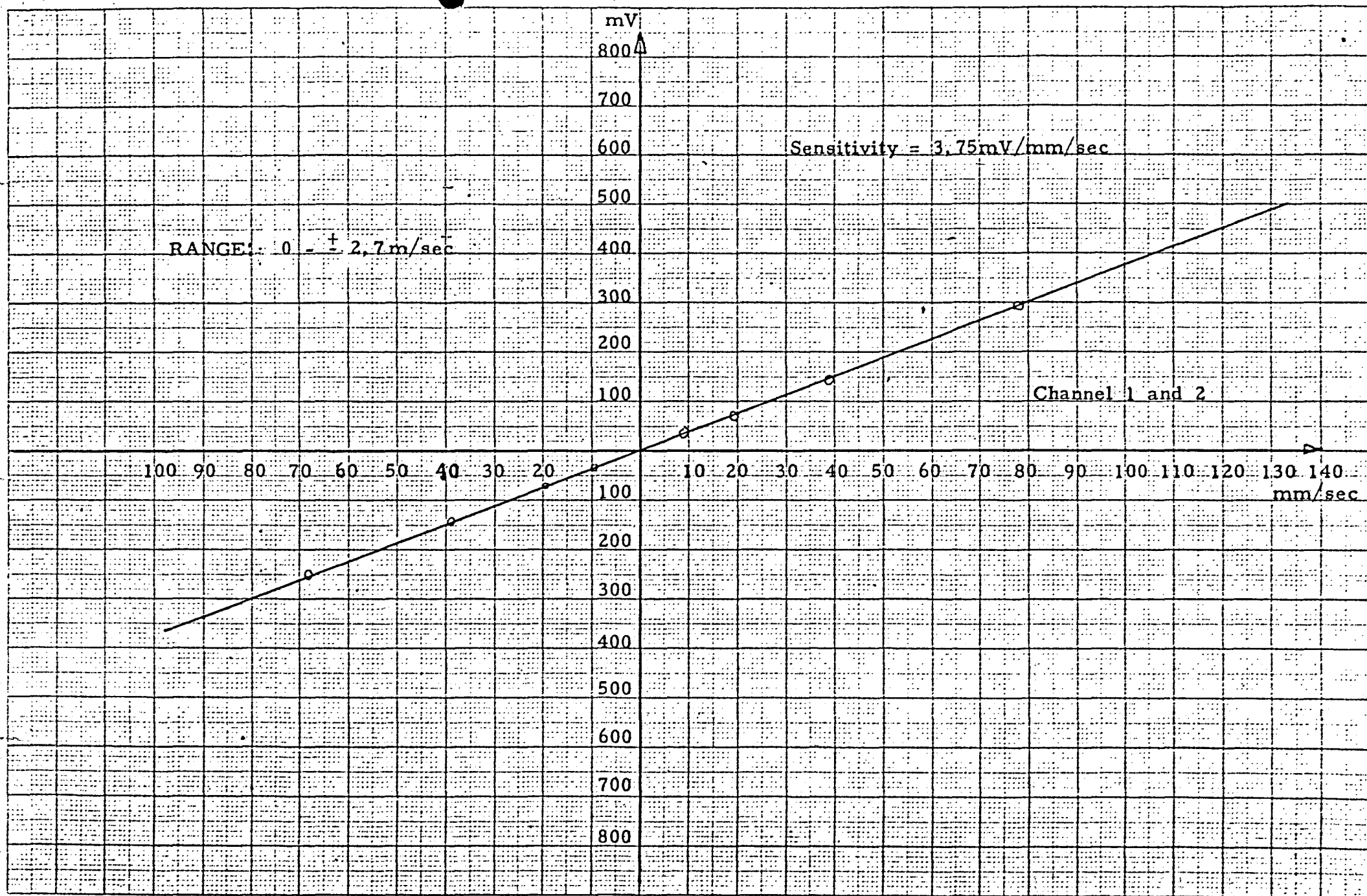
Fig. 5: Calibration curve
